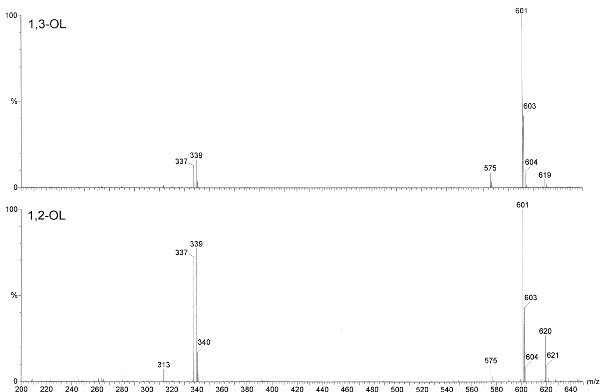
Fig. 7. Positive-ion APCI mass spectra of 1,3-oleoyl-linoleoyl-glycerol (1,3-OL) and 1,2-oleoyl-linoleoyl-glycerol (1,2-OL).
